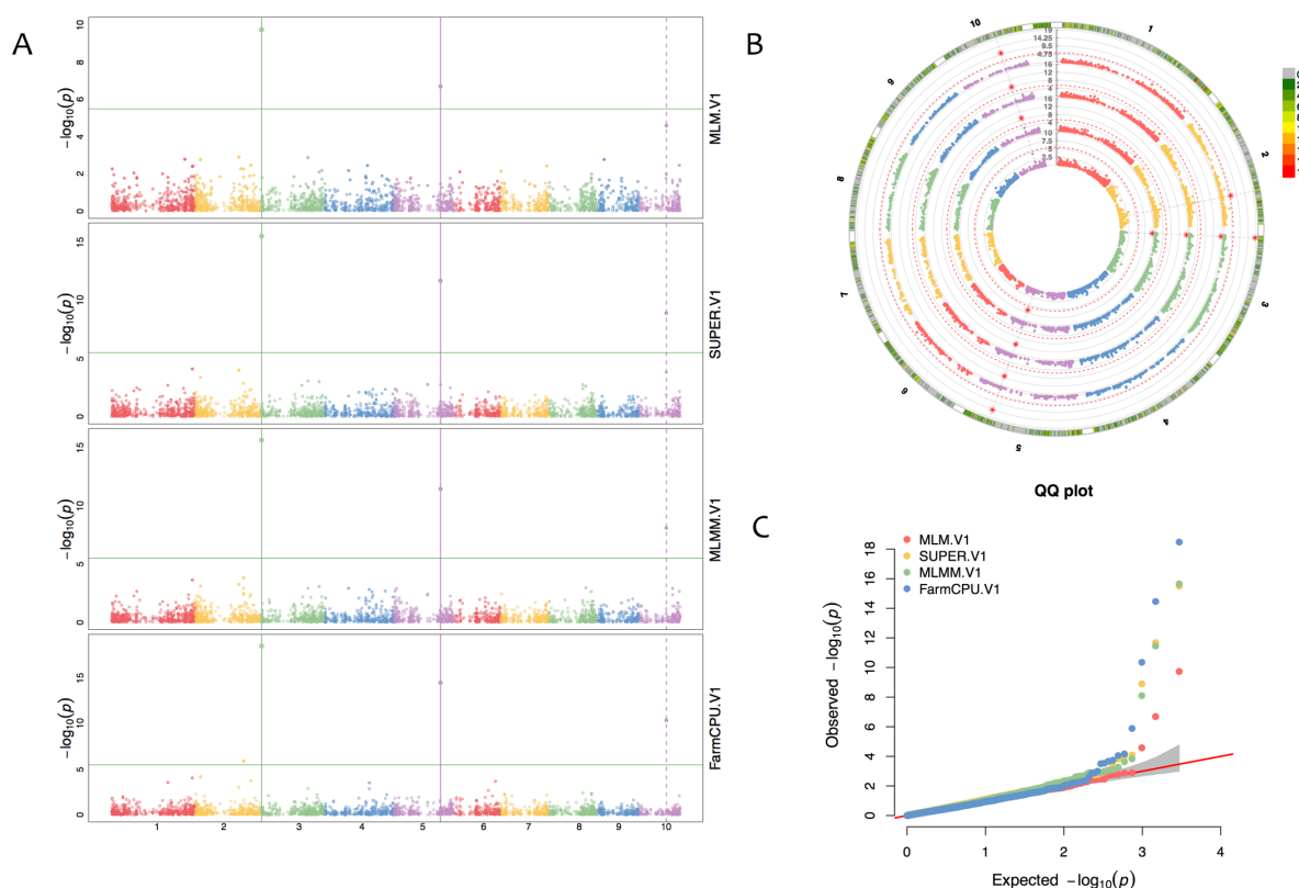
Figure 4.15.1 Multiple traits or methods Manhattan and QQ plot. The dash line in the Figure A indicated the common significant markers were detected by two methods or traits. The solid line in the Figure A indicated the common significant markers were detected by more than two methods or traits.
