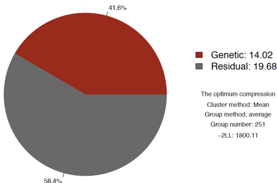
Figure 4.13.1 The profile for the optimum compression. The optimal method to calculate group kinship is “Mean”, the optimal clustering method is “average”, the number of groups (ie., the dimension of the group kinship matrix) is 251, the value of -2 \times \log likelihood function is 1800.11, and the heritability is 41.6%.
