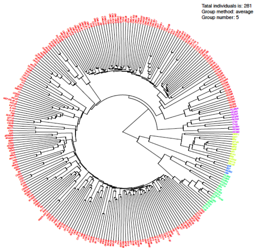
Figure 4.7.1 Neighbor-Joining (NJ)-tree The whole population was divided into 5 clusters with each colors.
