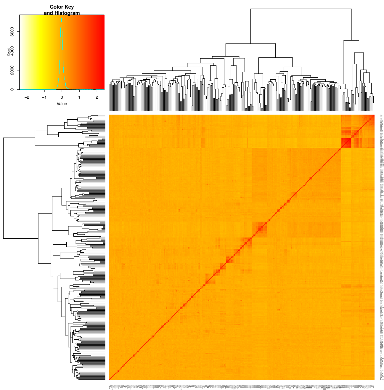
Figure 4.6.1 Kinship plot. A heat map of the kinship matrix is created to indicate the relationship between individuals.
